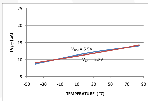
Figure 7. I_{BAT} vs. Temperature at V_{CC\_C}=1.8V ( V_{SEL}=LOW )
