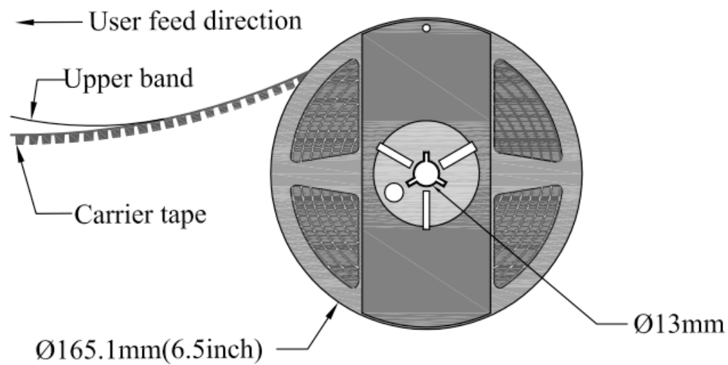
Figure 5. Reel dimensions.
