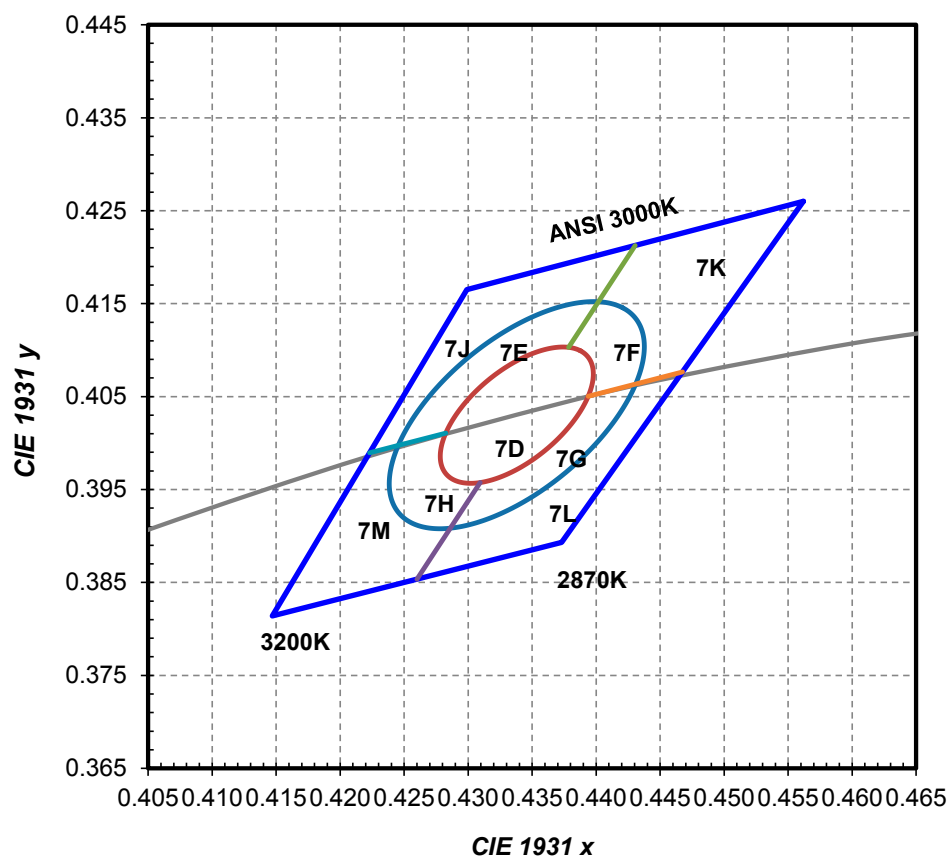
Figure 16. 3000K 1/9 th color bin structure.
