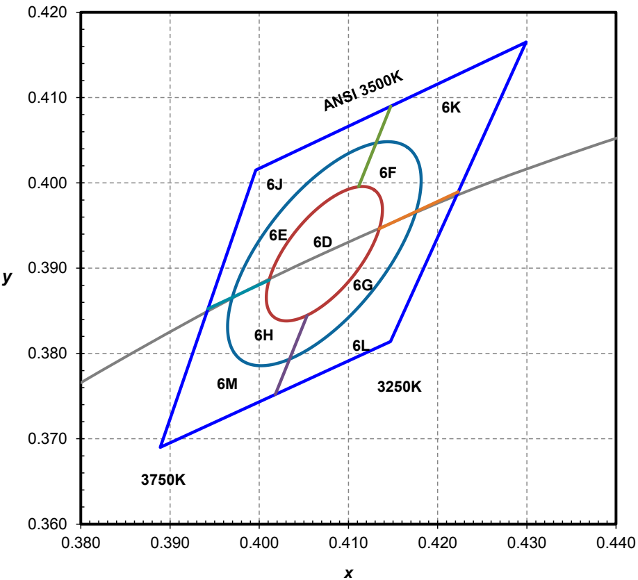
Figure 17. 3500K 1/9 th color bin structure.
