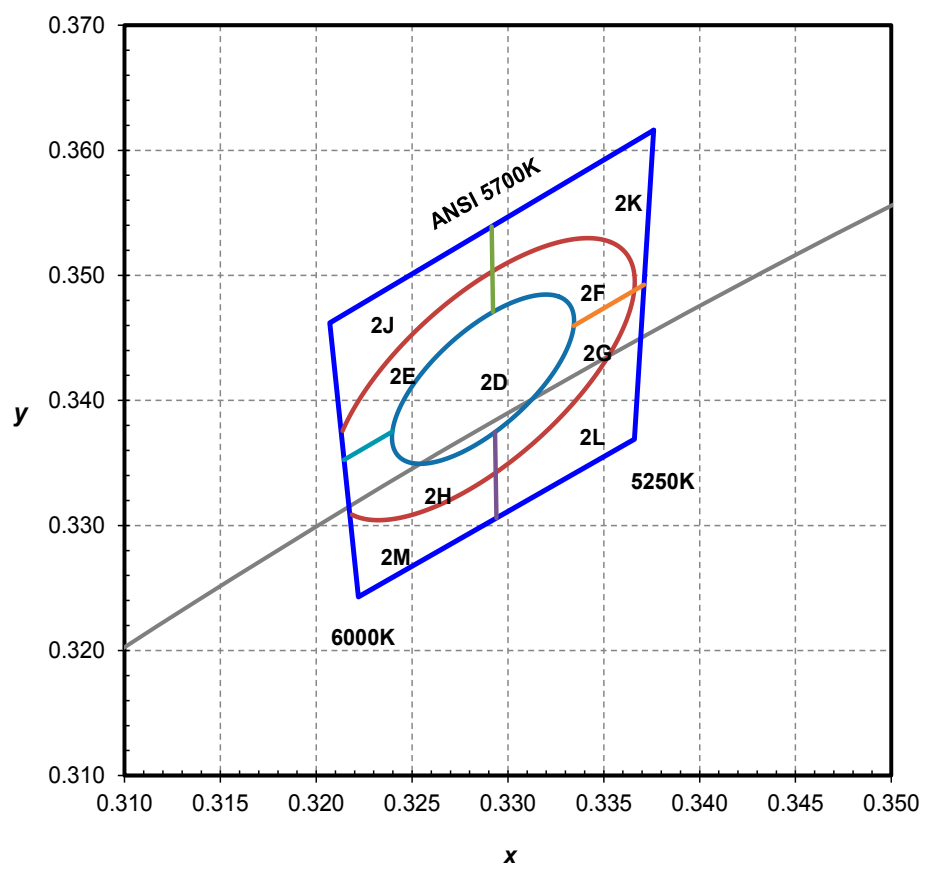
Figure 20. 5700K 1/9 th color bin structure.
