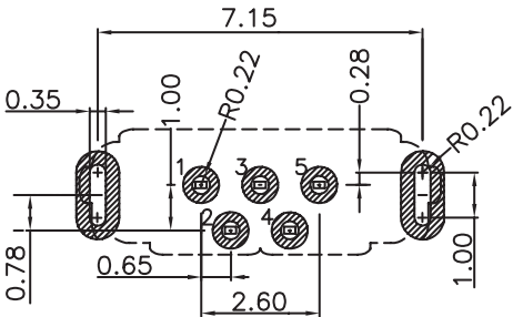
RECOMMENDED PCB LAYOUT RECOMMENDED PCB THICKNESS : 1.0 mm
