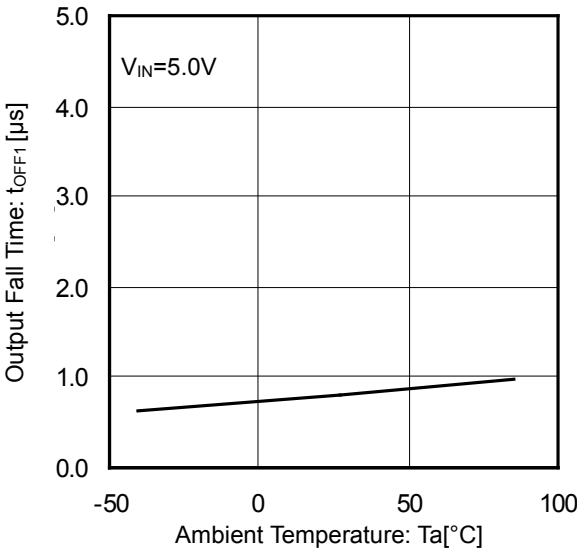
Figure 23. Output Fall Time vs Ambient Temperature
