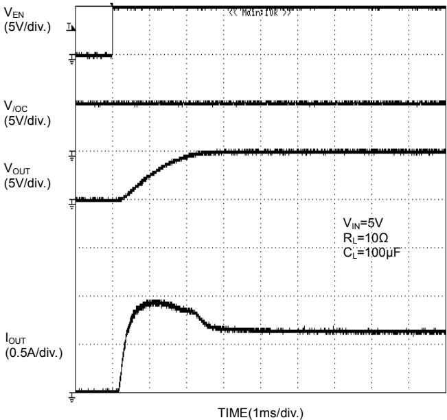
Figure 30. Output Rise Characteristic (BD2056AFJ)
