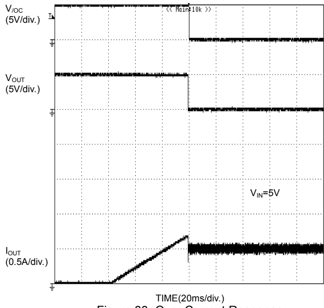
Figure 33. Over Current Response Ramped Load (BD2056AFJ)
