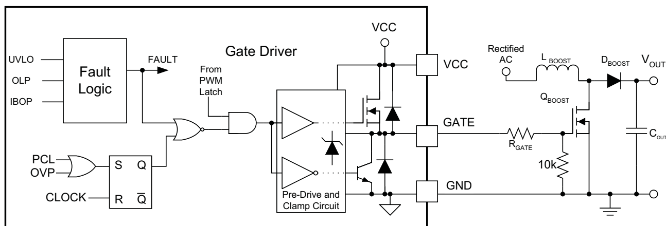
Figure 25. Gate Driver
