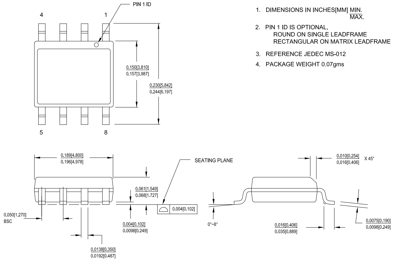
Figure 16. 8-pin SOIC (150 Mils) Package Outline, 51-85066
