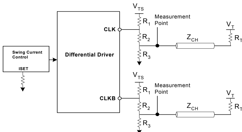
Figure 3. Clock Outputs
