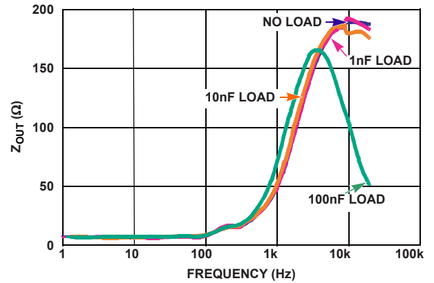
FIGURE 15. Z OUT vs FREQUENCY
