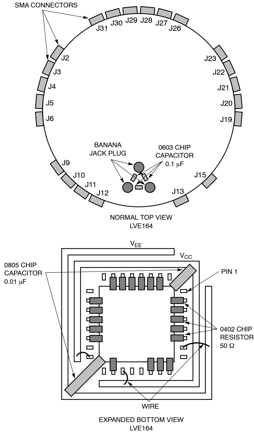
Figure 6. Configuration 1
