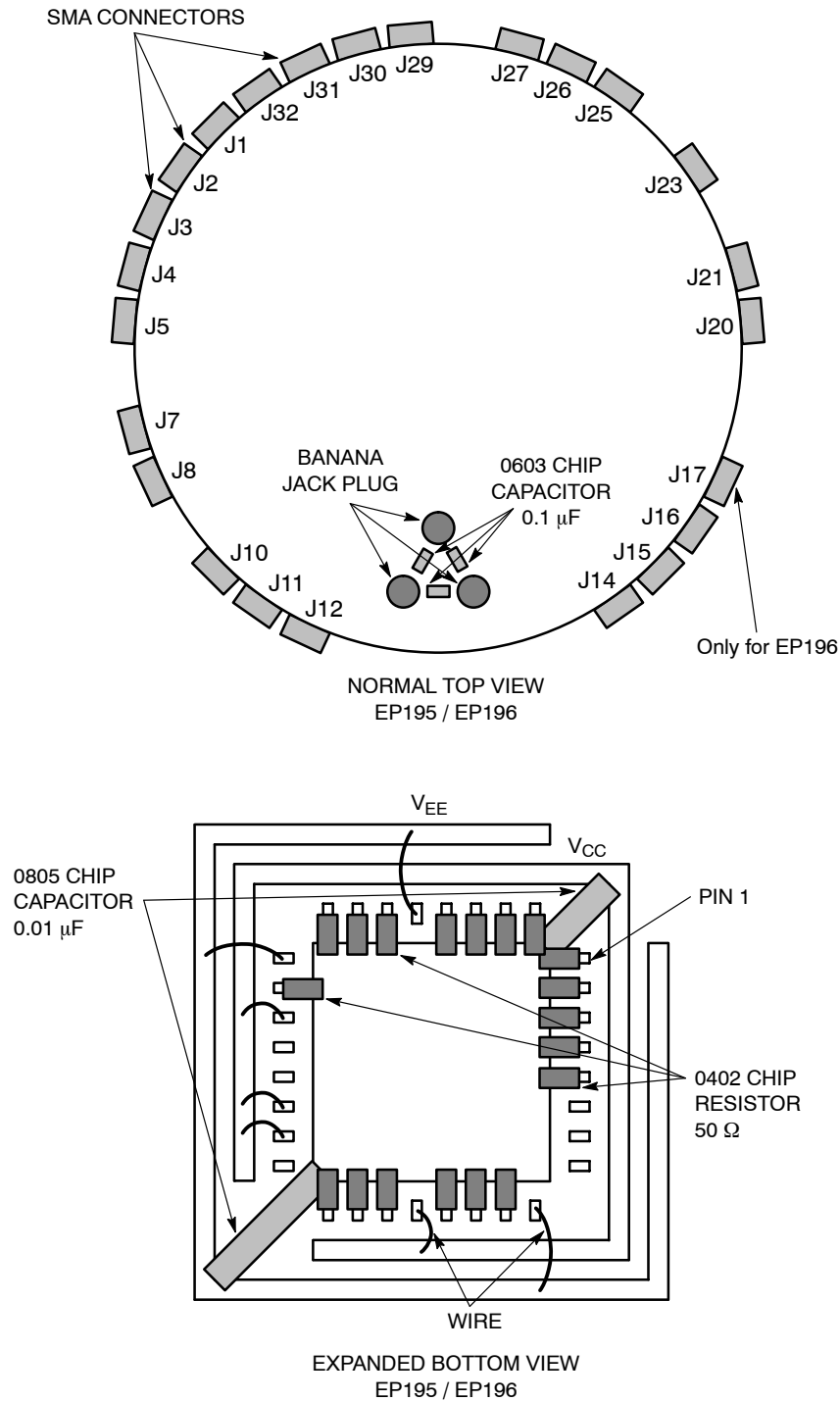
Figure 12. Configuration 7
