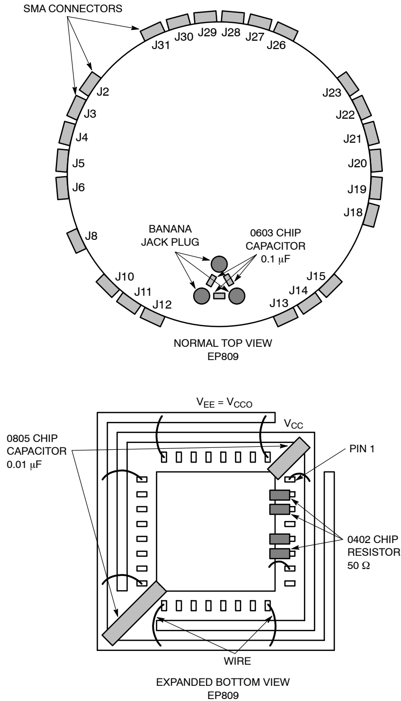
Figure 16. Configuration 11
