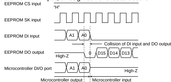
Figure 54. Collision timing at read data output at DI, DO direct connection
