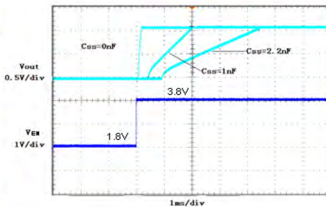
Figure 18 Turn-On Response
