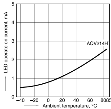
5-(2). LED operate current vs. ambient temperature characteristics
