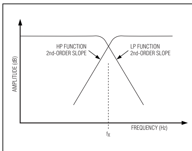
Figure 6. Crossover Frequency
