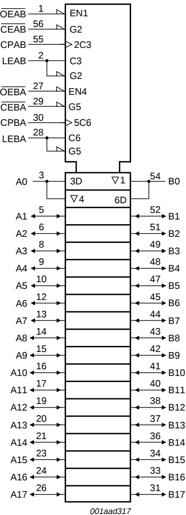
Fig 2. IEC logic symbol
