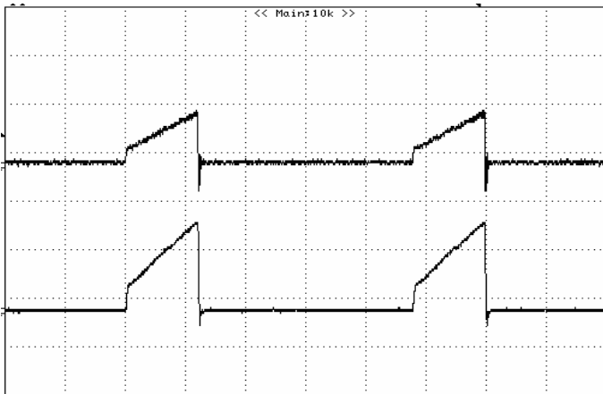
Figure 25: Typical transient response to step load change at 5A/μs from 25% to 75% of I_o , max at 12Vin, 3.3V out (Cout = 1μF ceramic, 10μF tantalum) Top: 100mV/div, 50μs/div, Bottom: 20A/div, 50μs/div
