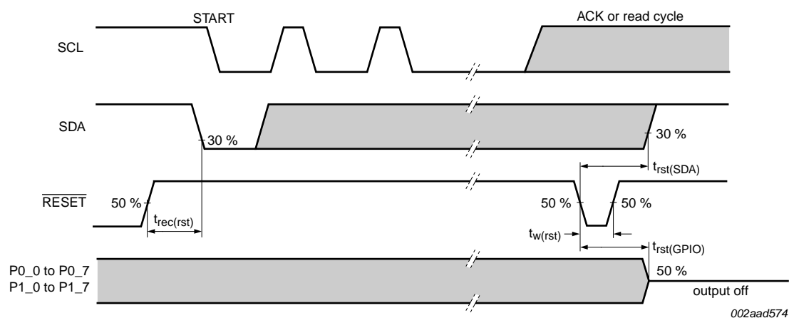
Fig 23. Reset timing
