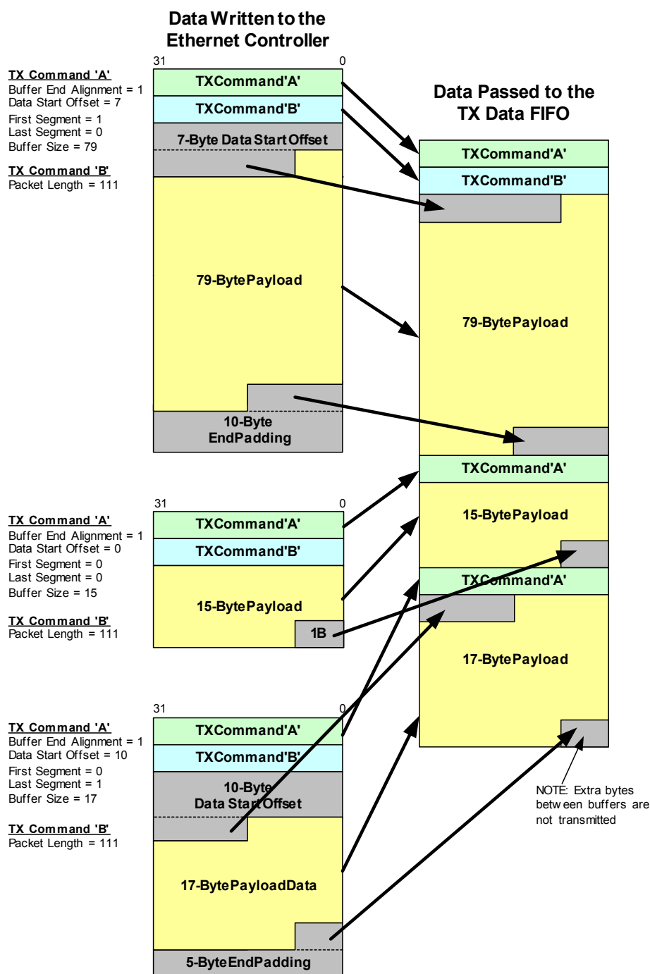
Figure 3.14 TX Example 1
