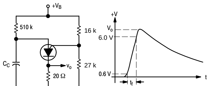
Figure 1. Electrical Characterization
