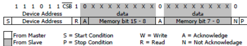
Figure 12: I 2 C answer from MS5803-02BA
