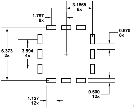
Figure 5. Second-Level Assembly Pad Layout
