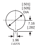
MOUNTING HOLE
