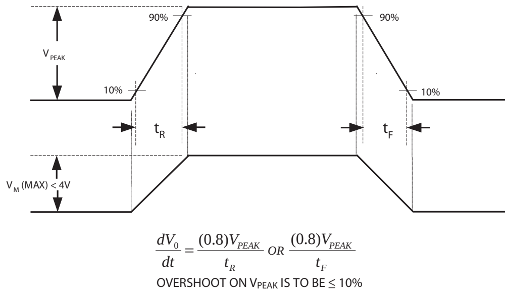
Figure 17. Output Transient Rejection Test Circuit
