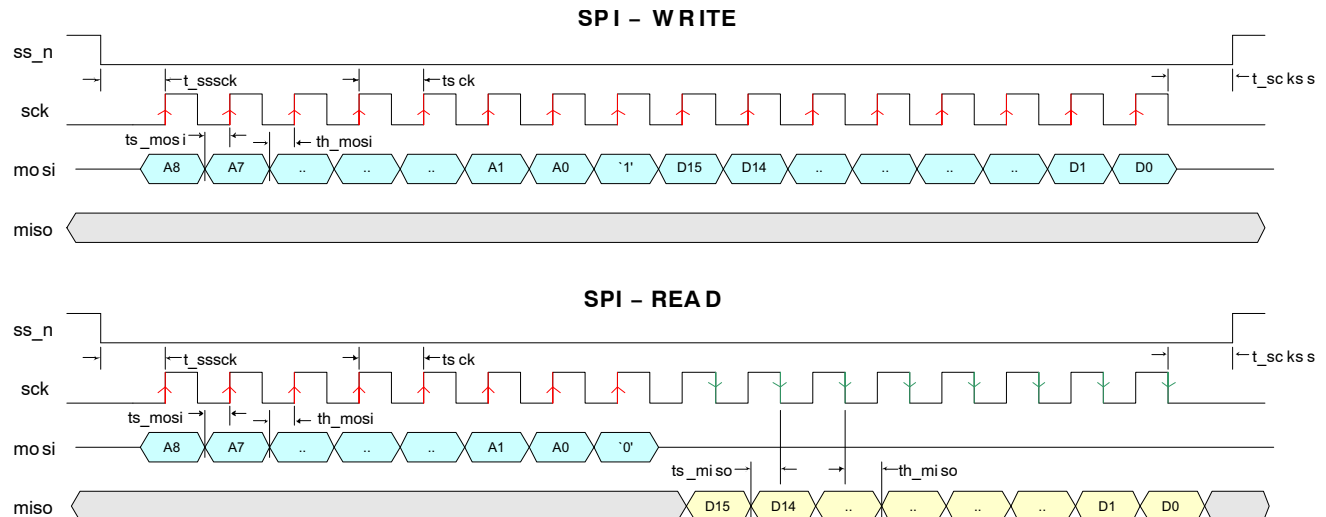
Figure 17. SPI Read and Write Timing Diagram
