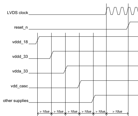
Figure 13. Power-up Procedure
