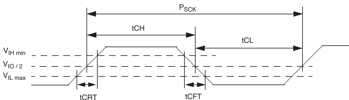
Figure 5.8 Clock Timing
