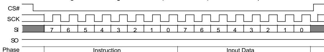
Figure 9.20 Program NVDLR (PNVDLR 43h) Command Sequence
