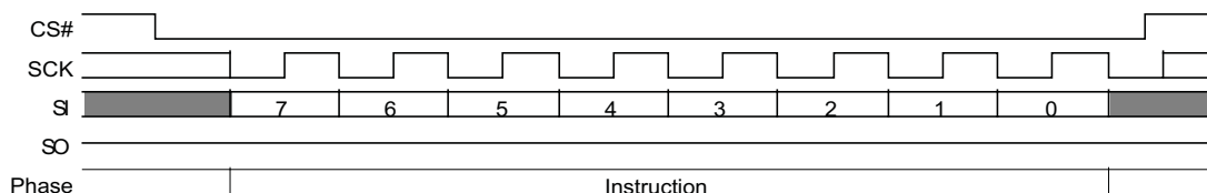
Figure 9.73 Software Reset (RESET F0h) Command Sequence
