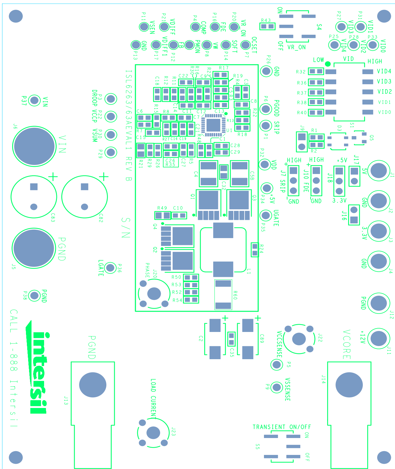
FIGURE 2. ISL6263AEVAL1Z AND ISL6263BEVAL1Z EVALUATION BOARDS PCB TOP SILKSCREEN
