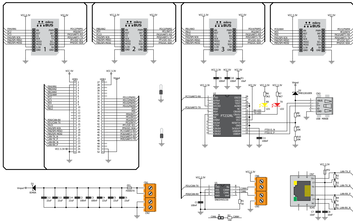
Figure 1-2: mikromedia+ shield schematic
