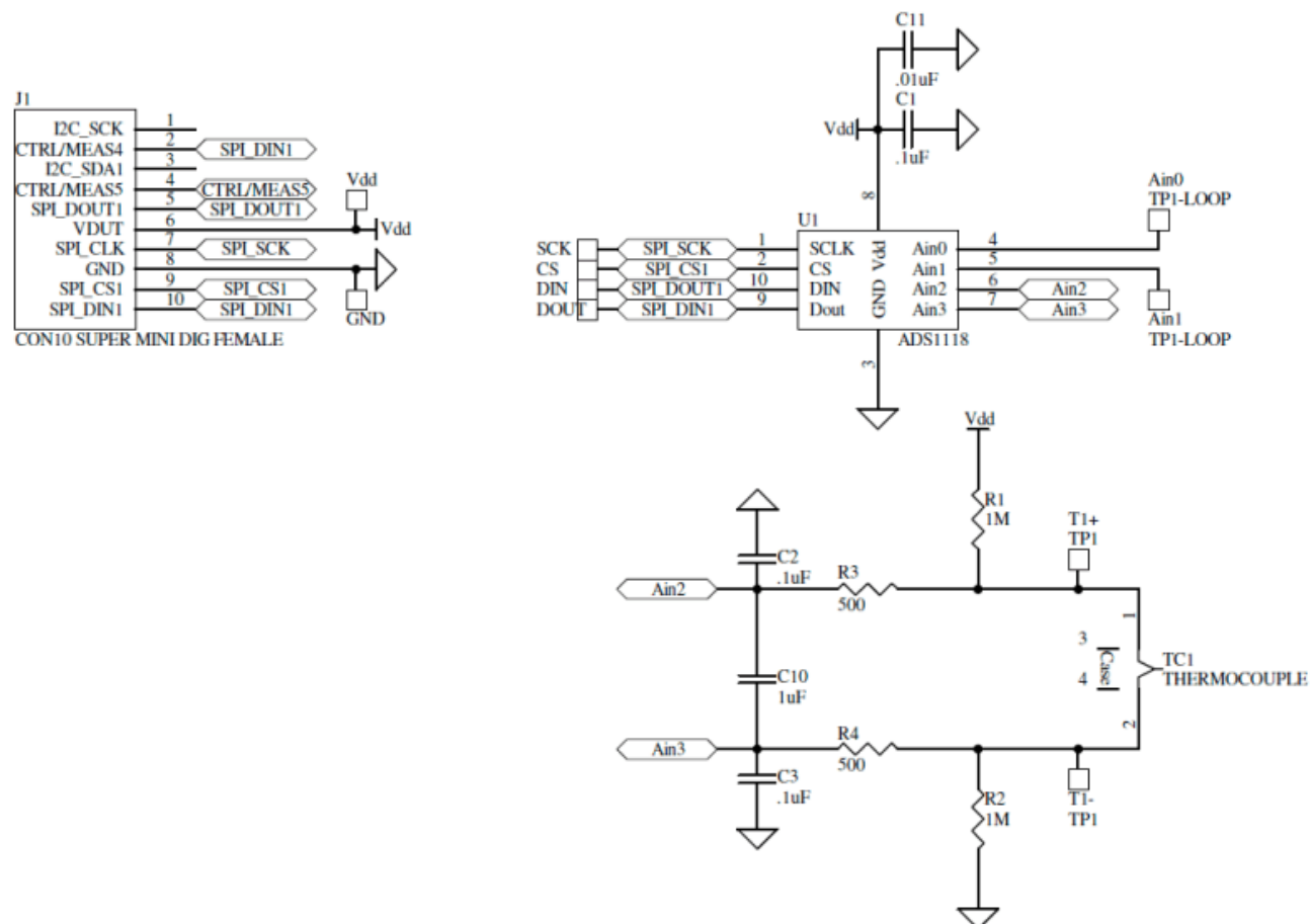
Figure 23. ADS1118EVM Schematic
