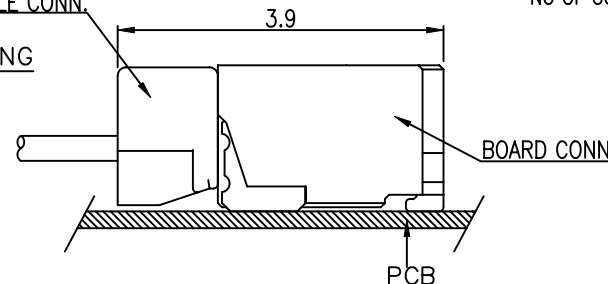
MATED CONDITION
