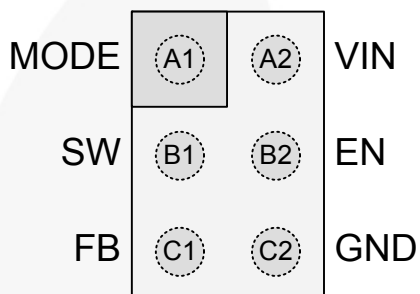
Figure 2. WLCSP, Bumps Facing Down
