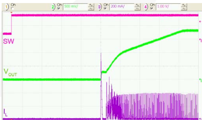
Figure 38. Soft-Start, R_{LOAD} = 50\Omega , 20\mu s/div.
