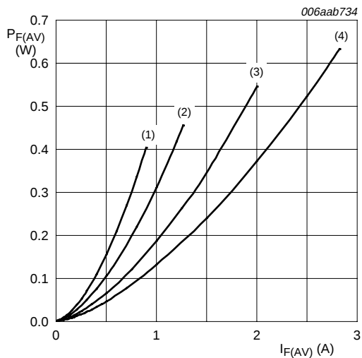
T_j = 150\text{ }^{\circ}\text{C} (1) \delta = 0.1 (2) \delta = 0.2 (3) \delta = 0.5 (4) \delta = 1
