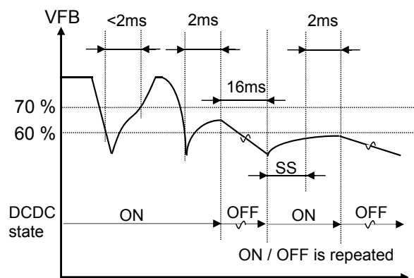
Note : SS = Soft start time Figure : SCP Operation1 PRTCNT = L / OPEN : Auto recovery case
