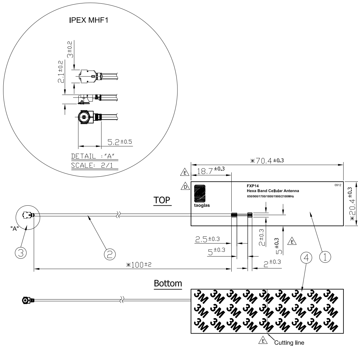
Figure 9. Mechanical Drawing for the FXP14 Antenna
