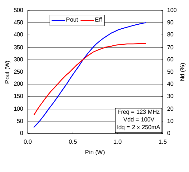
Figure 9. Pout and efficiency vs pin power 1 msec - 10 %
