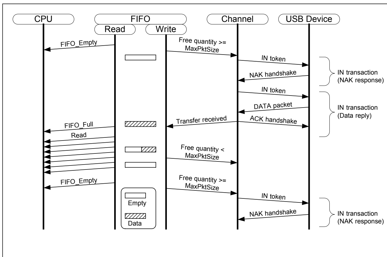
Figure 4-6: Typical data flow (with FIFO assigned for \text{MaxPktSize} and IN transfers)
