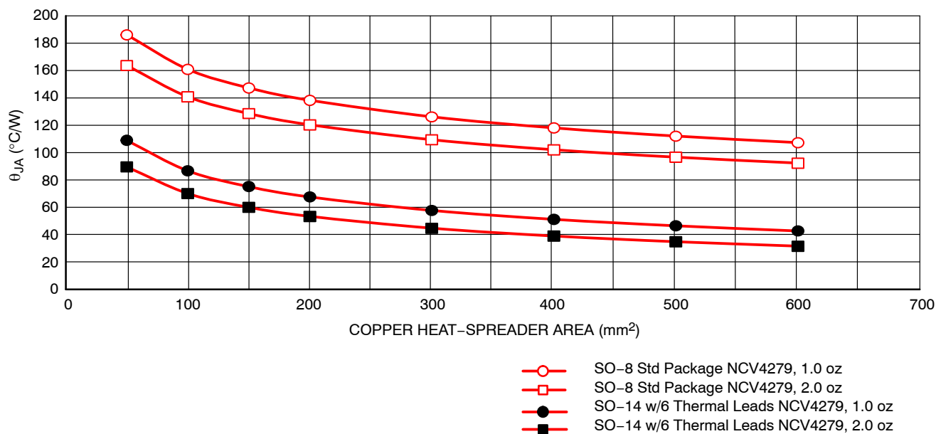
Figure 18. Junction-to-Ambient Thermal Resistance ( \theta_{JA} ) vs. Heat Spreader Area
