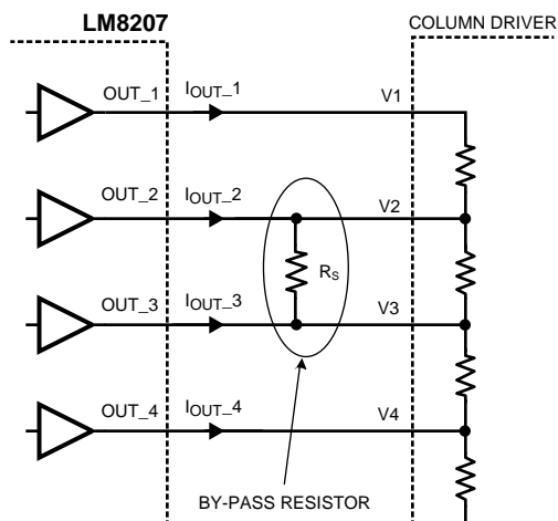
Figure 39. Using additional by-pass resistor to increase current sinking capability
