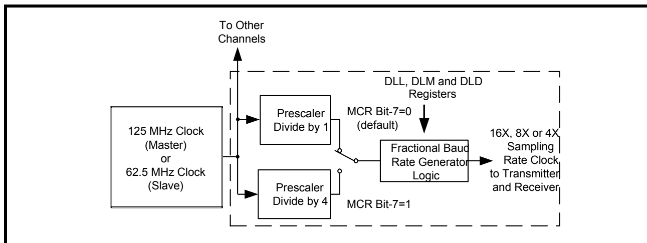
FIGURE 9. BAUD RATE GENERATOR
