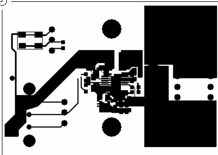
FIGURE 2: SP7648UEB PC LAYOUT TOP SIDE
