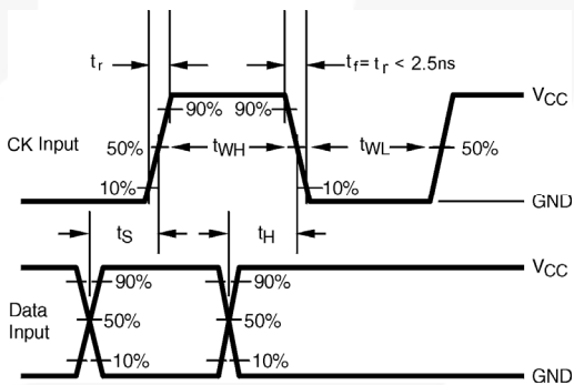
Figure 7. AC Waveforms
