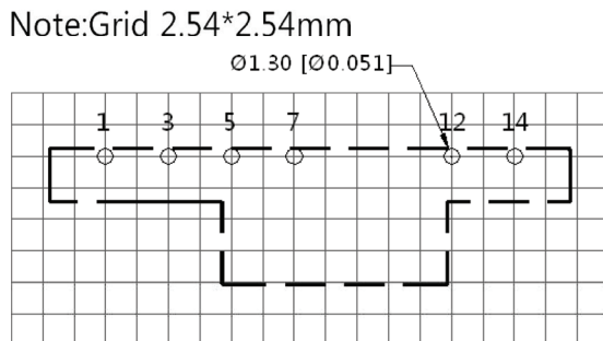
Top View PCB Layout
