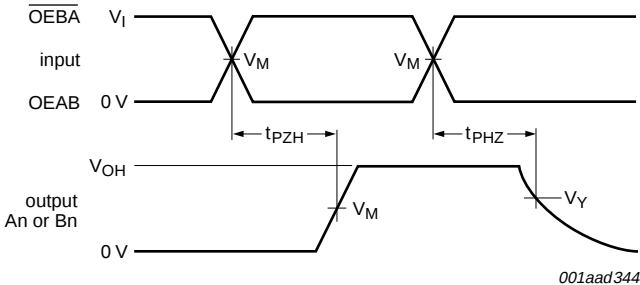
Measurements points are given in Table 8 . V_{OH} is typical voltage output drop that occur with the output load.
