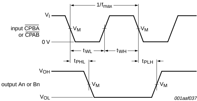
Measurements points are given in Table 8 . V_{OL} and V_{OH} are typical voltage output drop that occur with the output load.
