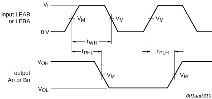
Measurements points are given in Table 8 . V_{OL} and V_{OH} are typical voltage output drop that occur with the output load.
