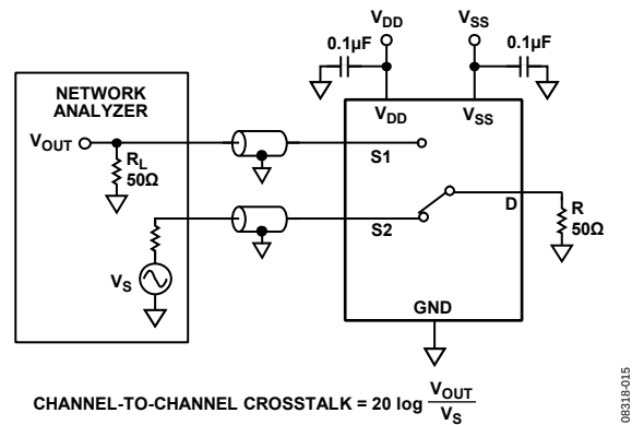
Figure 34. Channel-to-Channel Crosstalk
