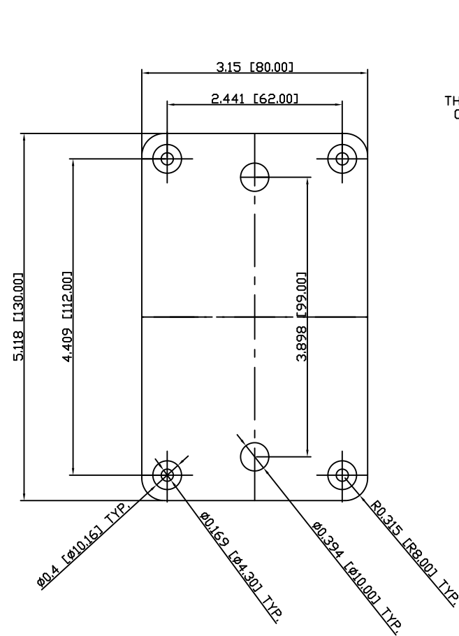
BOTTOM VIEW
