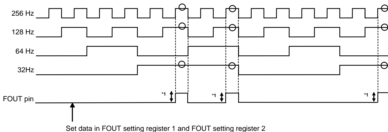
Figure 24 Example of output of clock pulse
