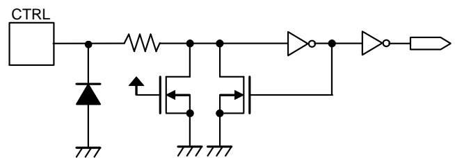
Figure 6 CTRL Pin
