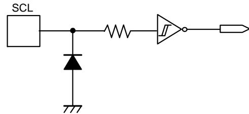
Figure 4 SCL Pin
