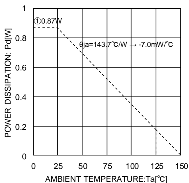
Figure 26. SSOP-B16 Power dissipation heat attenuation characteristics
