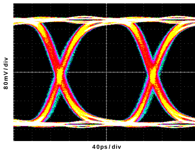
FIGURE 7. QLx4600-SL30 OUTPUT AFTER 12m OF 30AWG TWIN-AXIAL CABLE (CABLE B), 5Gb/s
