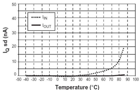
Fig. 14: Quiescent Current vs. Temperature. V_{IN} = 3.6V , SHDN = GND (Shutdown)
