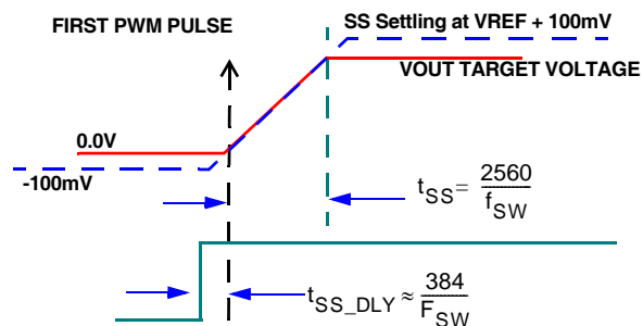
FIGURE 22. SOFT-START WITH VOUT = 0V
