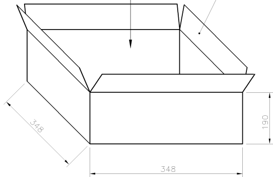
SHIPPING BOX
