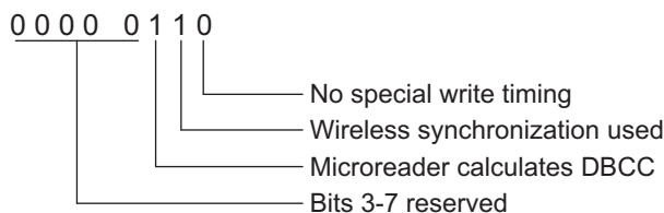
Figure 9. LMP Command Byte Field 2 Example
